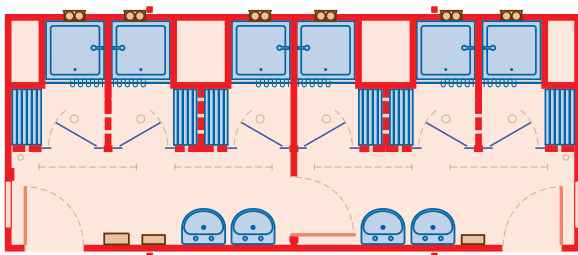
Typical layout of jackleg 24' x 10' male/female shower unit (3 + 3)
