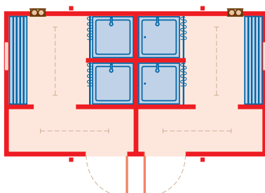
Typical layout of mobile gas-powered shower unit
