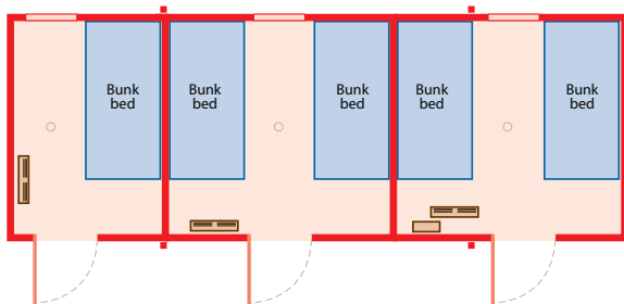
Typical layout of jackleg 24' x 10' Hospitality unit with kitchen
